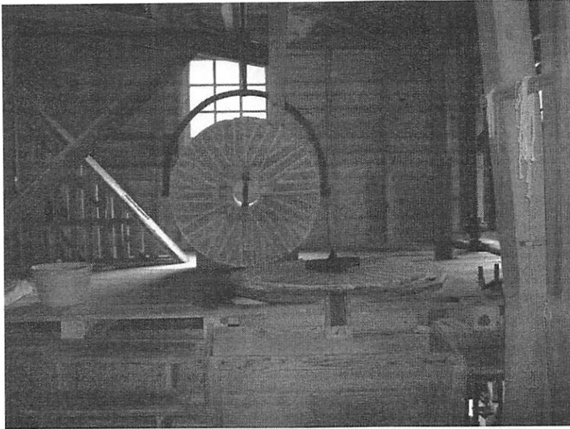
Figure 1: Quartzite millstones found inside Yates Mill. Notice the pattern carved into the stones. This pattern does the sheering, or cutting, of the corn kernels during the grinding process. When set up to grind, the upper, or runner stone, balances on the driving bar above the bottom, or bed stone. A case that is placed over the stones before the grinding process begins forces the meal to collect in the bin in the front of the picture.
